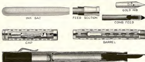
SECTIONAL VIEW
